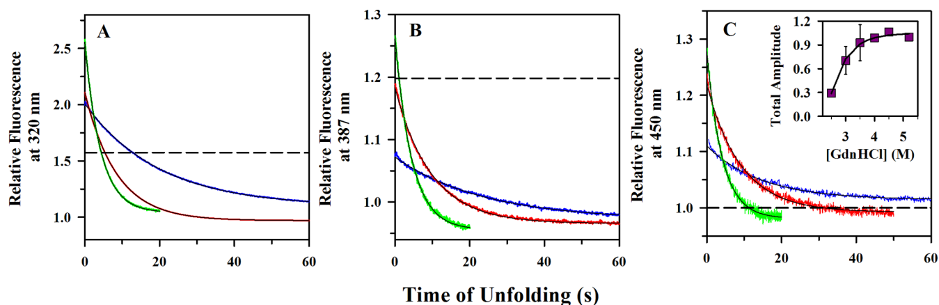
Figure 3. Kinetic traces of unfolding of the PI3K SH3 domain at pH 7.2 and 25 °C. Unfolding in GdnHCl was probed by measurement of the change in the intrinsic Trp fluorescence signal at 320 (A) and 387 nm (B), as well as of the change in ANS fluorescence at 450 nm with an excitation at 295 nm (C). The data in panels A–C were obtained when the native protein was diluted into 2.5 (blue), 3 (red), and 3.5 M GdnHCl (green). In panels A and B, each trace was normalized to a value of 1 for the fluorescence signal of the unfolded protein in 4 M GdnHCl. In panel C, each trace was normalized to a value of 1 for the fluorescence signal of the native protein. The inset in panel C shows the dependence of the total amplitude of the ANS fluorescence change (maroon squares) on the concentration of GdnHCl present during unfolding. The amplitudes are normalized to a value of 1 for the amplitude of the ANS fluorescence change observed for unfolding in 5.3 M GdnHCl. The dashed lines in panels A and B represent the fluorescence signal of the native protein. In all the panels, the solid lines through the traces represent fits to a single-exponential equation. The error bars represent standard deviations obtained from two independent experiments.
